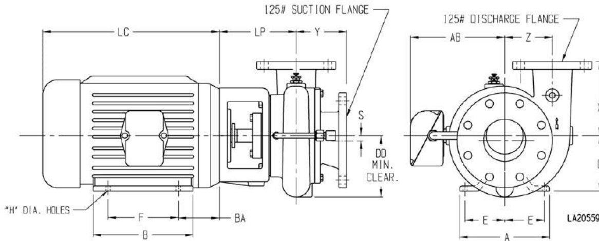
PUMP DIMENSIONS
